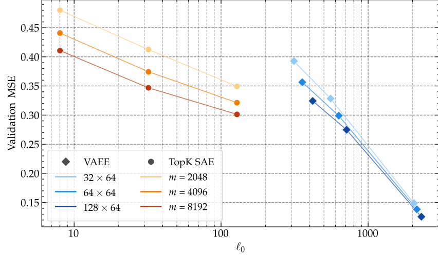
Figure 4.2: The sparsity–reconstruction frontier in active neurons \ell_0 , the decoder-capacity unit, over the same sweeps as fig. 4.1 — the SAE over k \in \{8, 32, 128\} and the VAEE over \tilde{\kappa} = \pi K \in \{4, 8, 32\} . The families occupy disjoint ranges — SAEs below \ell_0 = 128 , VAEs above \ell_0 \approx 300 — so no matched- \ell_0 comparison is available; the SAE reaches a given error with fewer active neurons.
